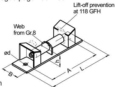
Type 118 GFH Roller bearing with lateral guide and lift-off prevention can be used in combination with glide support Type 180 HS / catalogue page 120 and Type 171-..HS / catalogue page 159+160
