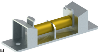
Type 118 GFH Roller bearing with lateral guide and lift-off prevention can be used in combination with glide support Type 180 HS / catalogue page 120 and Type 171-..HS / catalogue page 159+160
